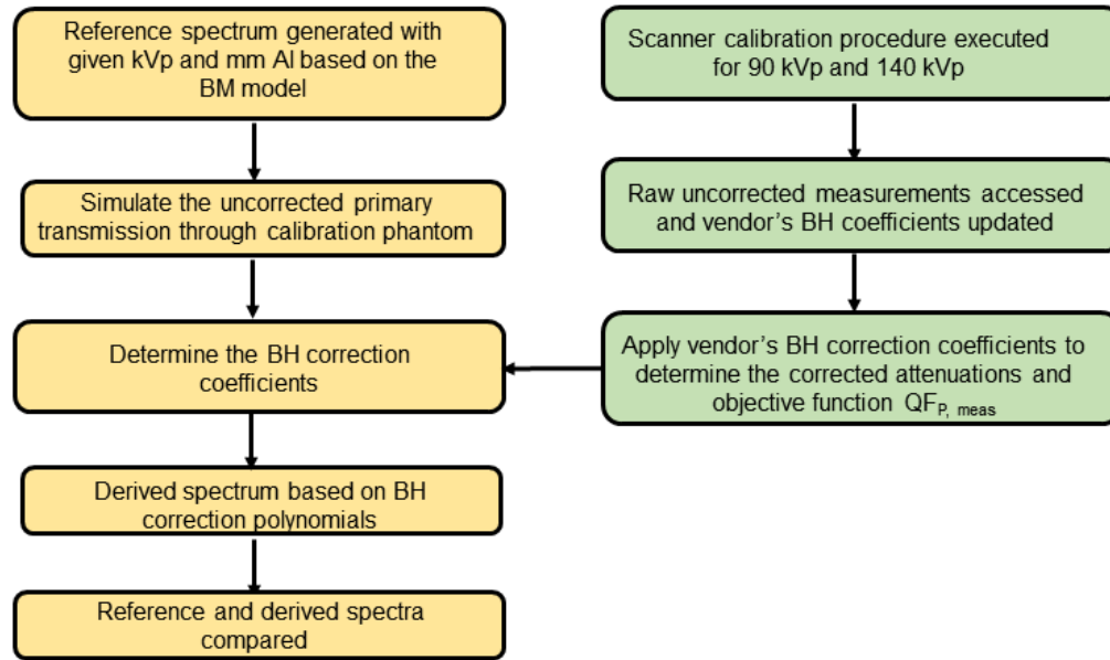
Fig.4.8. Flowchart of the procedure of robustness analysis of spectrum. Given a wide range of variations of spectral parameters, the robustness analysis compares the reference and derived spectra for each pair of parameters
