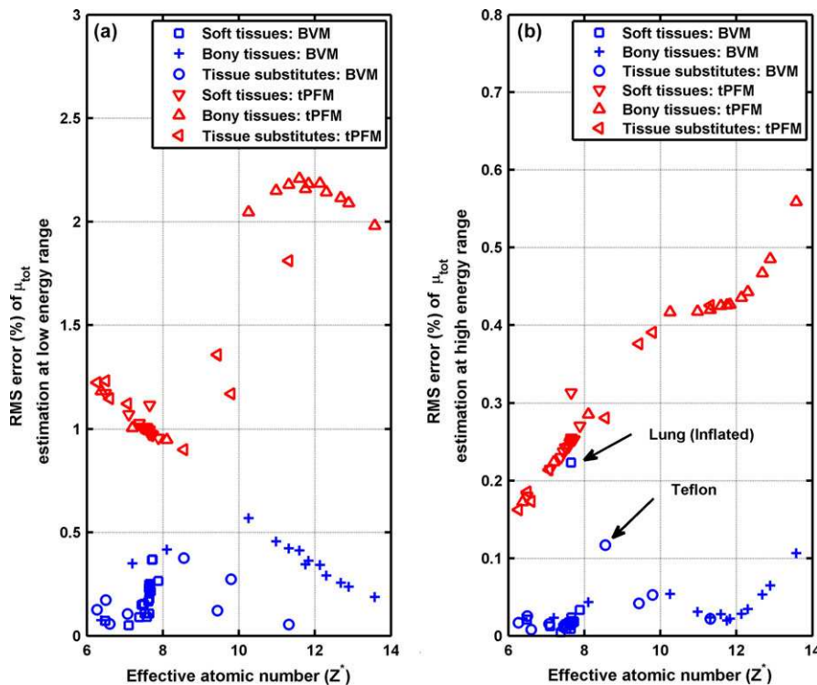
FIG. 1. Percent RMS error of the total linear attenuation coefficient predicted by BVM or tPFM for 43 tissues and phantom substitutes as functions of tPFM effective atomic number for the (a) 20 \leq E \leq 50 keV and (b) 50 \leq E \leq 1000 keV energy ranges. The thyroid tissue prediction error is outside the plotting range of the low-energy plot. [Color figure can be viewed at wileyonlinelibrary.com]
