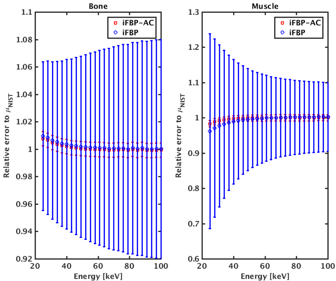
Fig. 5.17 Mean errors with 95% uncertainties error bars in estimated linear attenuation coefficient of ICRU bone and muscle tissue are shown for both iFBP and iFBP-AC algorithms, respectively.
