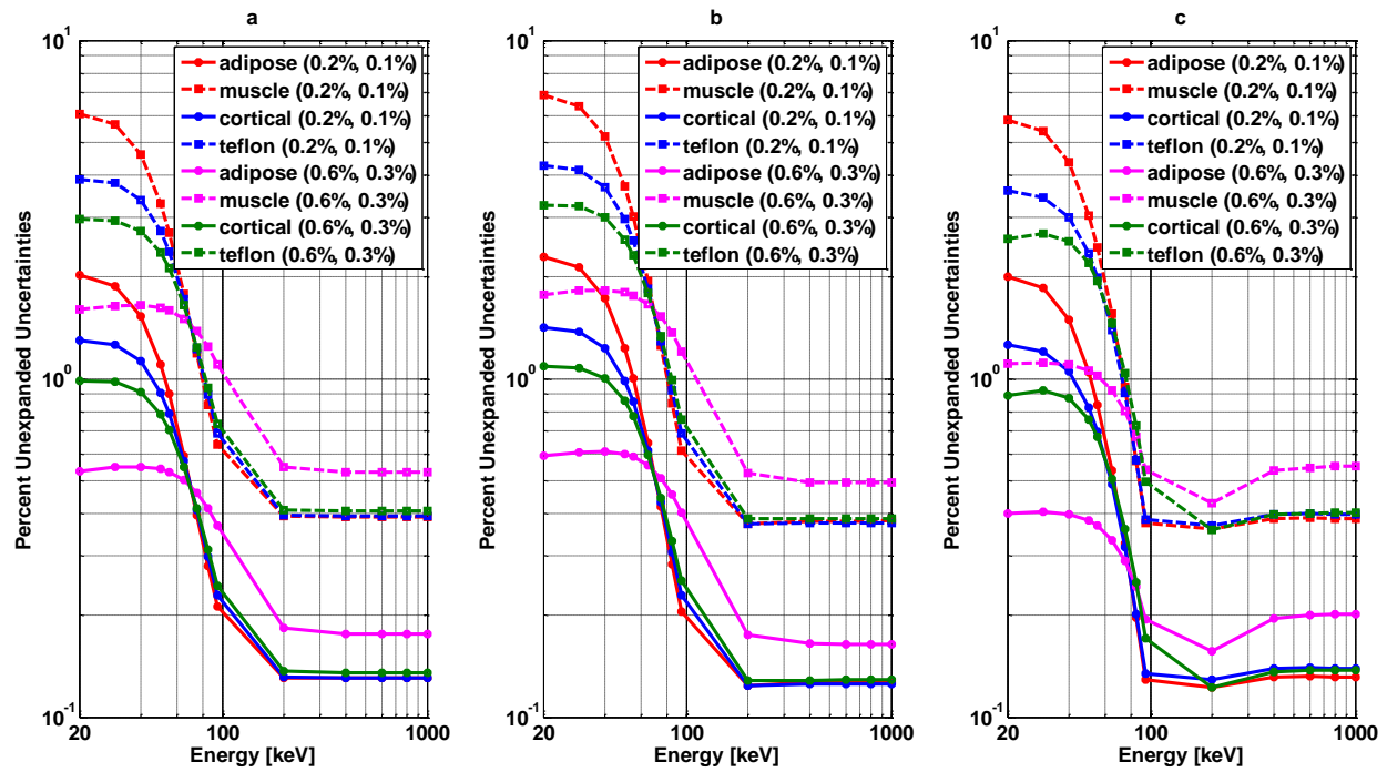
Figure S-F3. Percent unexpanded uncertainty of energy absorption coefficients for (a) tPFM, (b) vPFM and (c) BVM, respectively as functions of energy in the range 20 \leq E \leq 1000 keV, at image intensity uncertainty levels (0.6%, 0.3%) and (0.2%, 0.1%) for (low, high) energy CT images. Four typical human tissues and tissue substitute were selected for analysis.
