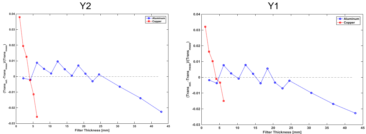
Fig. 4.11. The transmission comparisons for spectra of 90 kVp at Y1 and Y2 through Al and Cu filters
