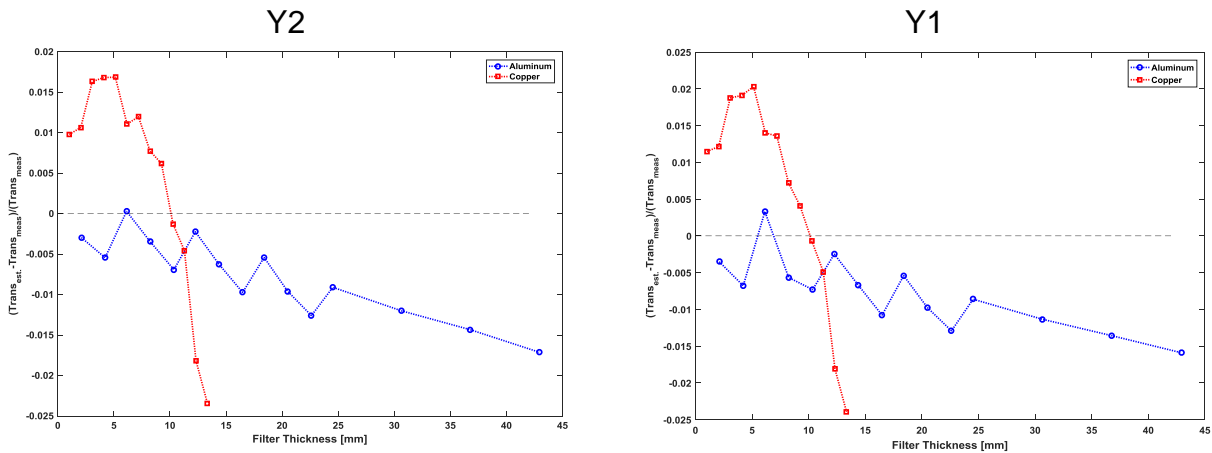
Fig. 4.12. The transmission comparisons for spectra of 140 kVp at Y1 and Y2 through filters
