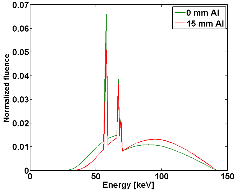
Fig. 4.1 Two normalized 140 kVp spectra penetrated aluminum plates with thickness of 0 mm and 15 mm, respectively
