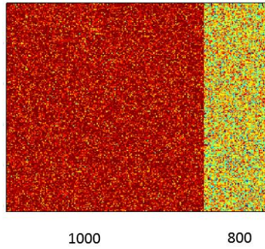
Fig.5.19. A synthetic image with 10% noise is shown. The contrast of two compartments is set 5:4
