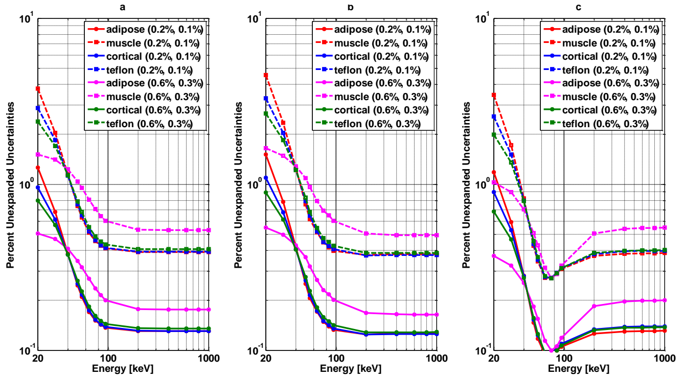
Figure S-F1. Percent unexpanded uncertainty of total linear attenuation for (a) tPFM, (b) vPFM and (c) BVM, respectively as functions of energy in the range 20 \leq E \leq 1000 keV, at image intensity uncertainty levels of (0.6%, 0.3%) and (0.2%, 0.1%) for (low, high) energy CT images. Four typical human tissues and tissue substitute were selected for analysis.
