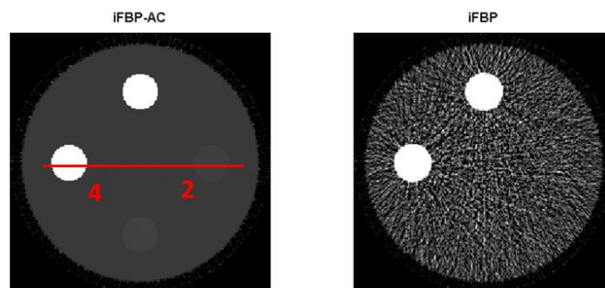
Fig. 5.13 Reconstructed c_2 images from noisy sinogram. A profile line across inserts 2 and 4 is shown. The noise levels in BVM muscle insert 2 for iFBP-AC and iFBP are 0.0012 and 0.077, respectively. The true c_2 value of insert is 0.13. The view window is set [0 0.2]
