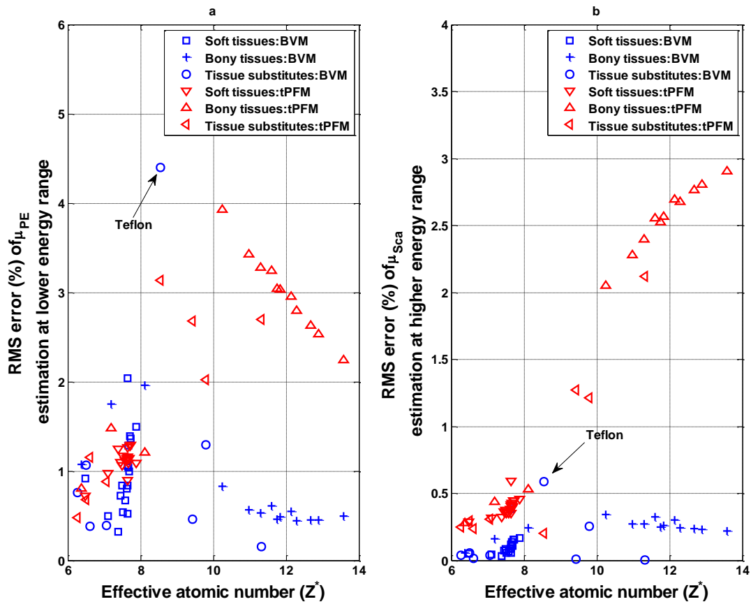
Fig 3.2 tPFM and BVM percent RMS predictions for 43 tissues and phantom substitutes as functions of tPFM effective atomic number for (a) photoelectric effect cross sections in the 20 \leq E \leq 50 keV range and (b) photon scattering cross sections in the 50 \leq E \leq 1000 keV range. The thyroid tissue prediction error is outside the plotting range of the low energy plot.
