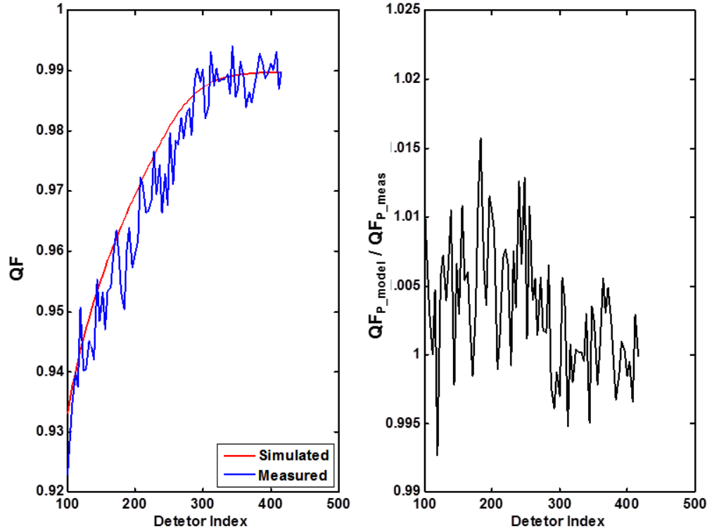
Fig.4.22. Comparison between QF_{P,model}(\gamma|\mathcal{B}_{Y_2}) and QF_{P,meas}(\gamma|\mathcal{B}_{Y_2}) for detector range [100,418] in
