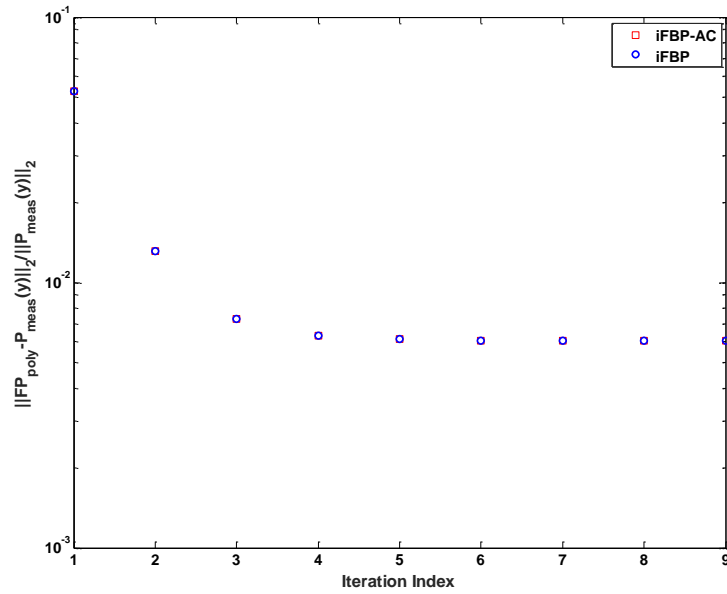
Fig.5.18 Relative difference between estimated and measured projections as a function of iteration
