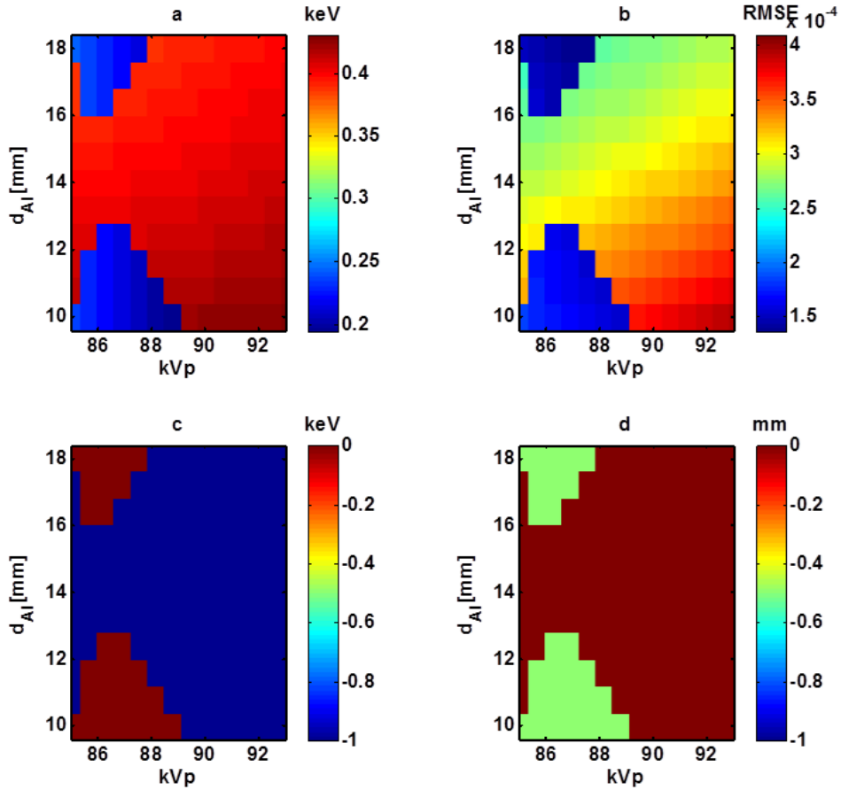
Fig.4.18 Comparisons of derived spectrum and independently simulated reference spectra for nominal 90 kVp with inherent filtration of aluminum ranging from 10 mm to 18 mm for the noisy QF_{P,model} . The differences of mean energy (a), RMSE (b), kVp(c), and d_{Al} (d) are shown, respectively. Each pixel on the figures corresponded to the discrepancy for each candidate of reference spectrum
