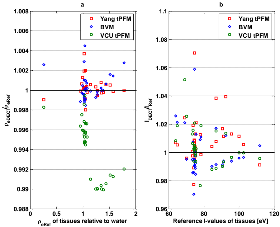
Fig. 2.4. The ratio of electron density and I-values estimation by three different models: the Yang tPFM, BVM, and VCU tPFM, respectively, to the reference value of stopping power. (a) Electron density and (b) I-values. The reference electron density of tissues is shown in the form of electron density relative to water. The reference I-values were computed based on the Bragg additivity rule.
