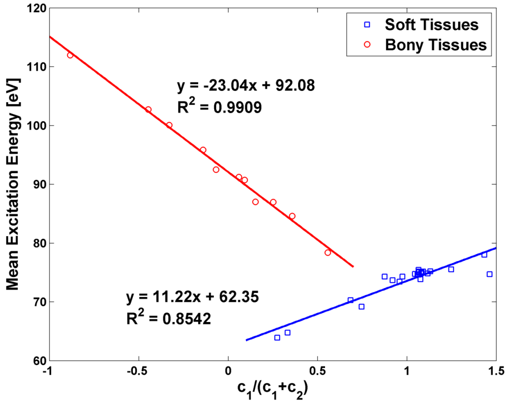
Fig. 2.2. The relationship between c_1/(c_1+c_2) and the I-values of 34 standard human tissues is shown. There are two separate linear fits, one for soft tissues and one for bony tissues. This relationship provides an alternative method to estimate I-value without knowing the Z^* of the substances. It was found the goodness of fit ( R^2 ) had minor impact on the achieved accuracy of proton stopping power estimation.
