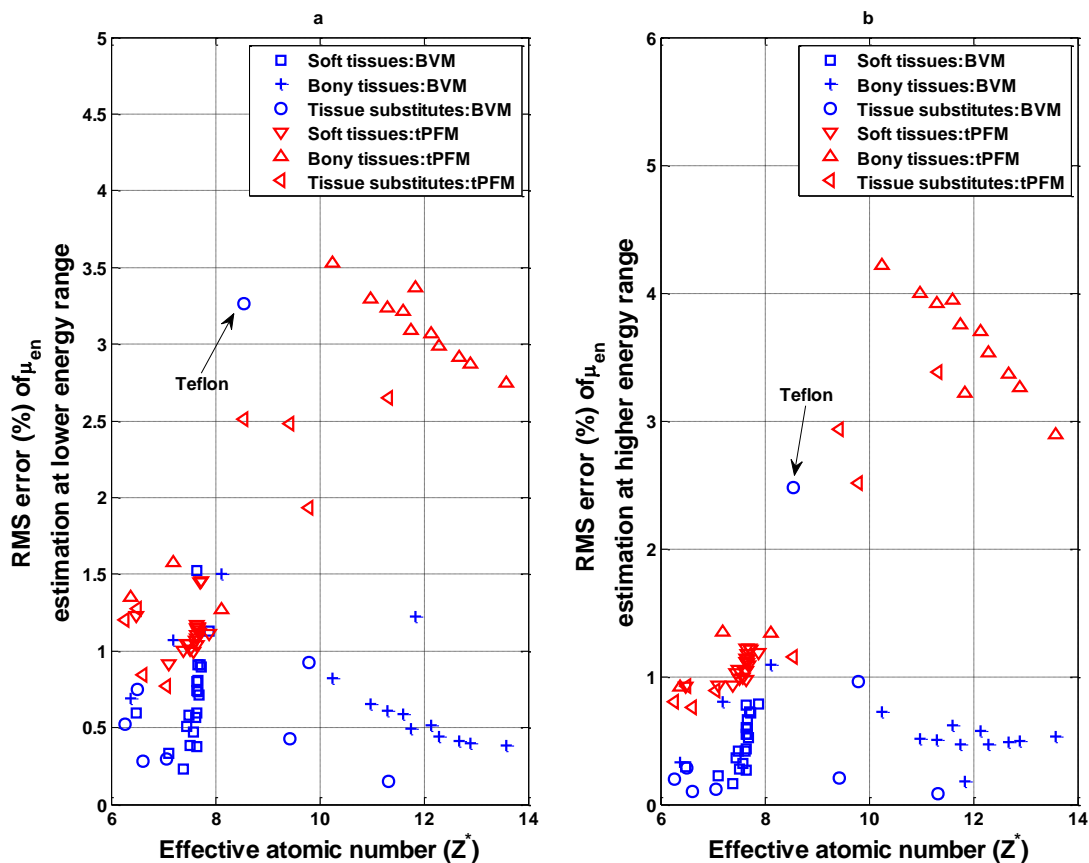
Fig 3.3. Percent RMS error of energy-absorption coefficients estimate for 43 tissues and phantom materials as functions of tPFM effective atomic number for the (a) 20 \leq E \leq 50 keV and (b) 50 \leq E \leq 1000 keV energy ranges. The thyroid tissue prediction error is outside the plotting range of the low energy plot
