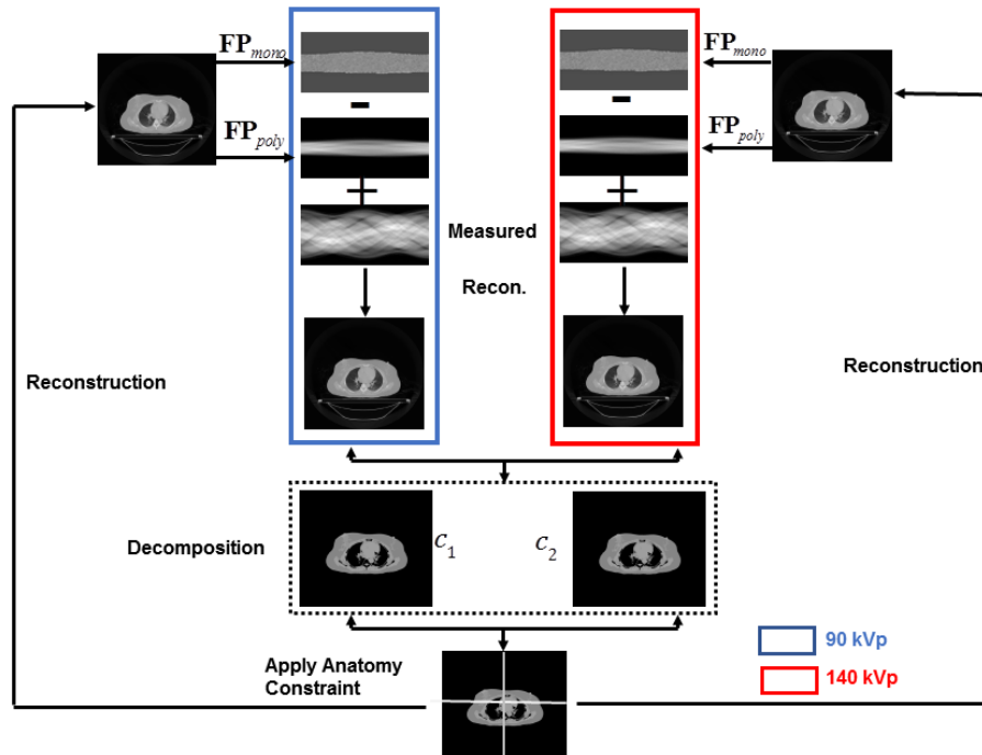
Fig. 5.3 illustration of iterative process of pseudocode of iFBP-AC
