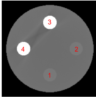
Fig. 5.5 Digital phantom of four inserts reconstructed with conventional FBP of OCCT software. The streaks are visible between two high density bones. The window is set [0.01, 0.03]
