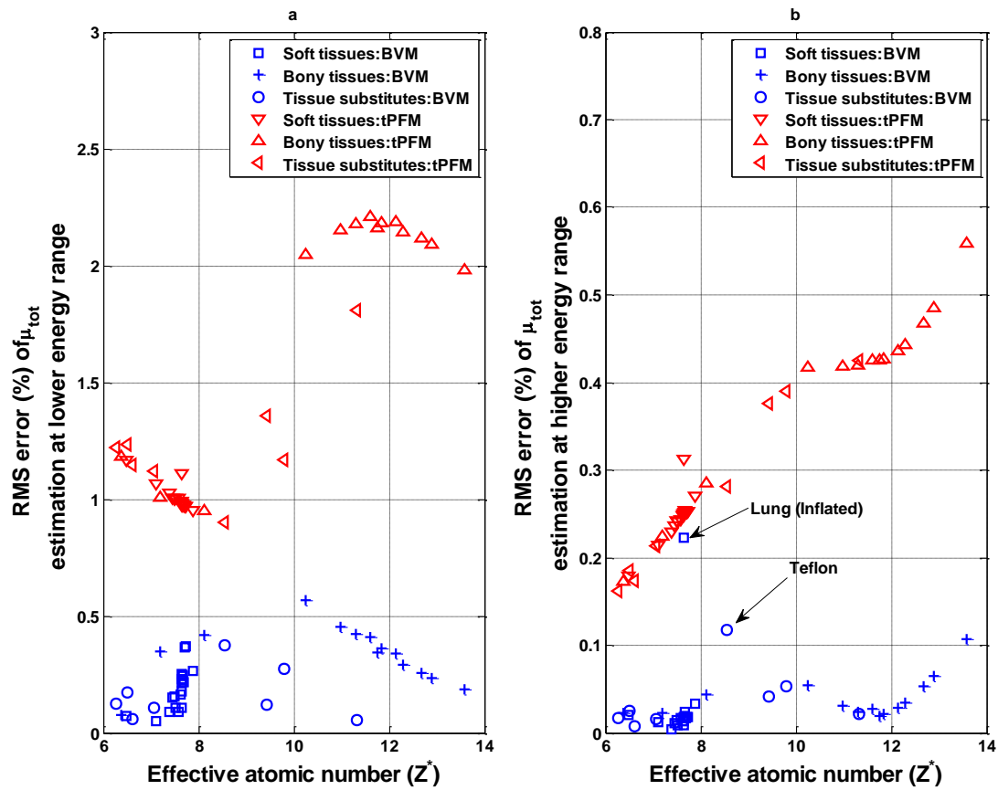
Fig. 3.1. Percent RMS error of the total linear attenuation coefficient predicted by BVM or tPFM for 43 tissues and phantom substitutes as functions of tPFM effective atomic number for the (a) 20 \leq E \leq 50 keV and (b) 50 \leq E \leq 1000 keV energy ranges. The thyroid tissue prediction error is outside the plotting range of the low energy plot.
