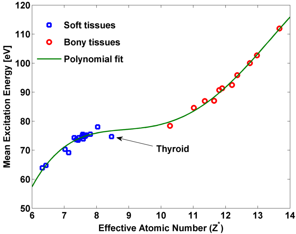
Fig.2.3 The polynomial relationship 55 between Z^* and mean excitation energy was implemented in the VCU tPFM. The fit of R^2 is 0.9603. Data for 34 soft tissues and bony tissues are shown.
