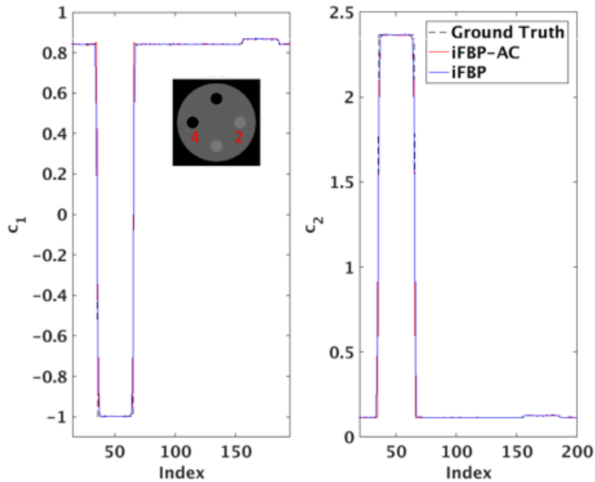
Fig 5.8 Profiles of component images along the red lines through inserts 2 and 4 from above images are shown. The ground truth c-values of components from BVM tissues are also shown.
