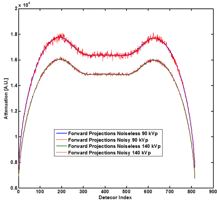
Fig.4.17 Comparisons of forward projections with and without noise for full calibration phantom at spectra of 90 kVp and 140 kVp.
