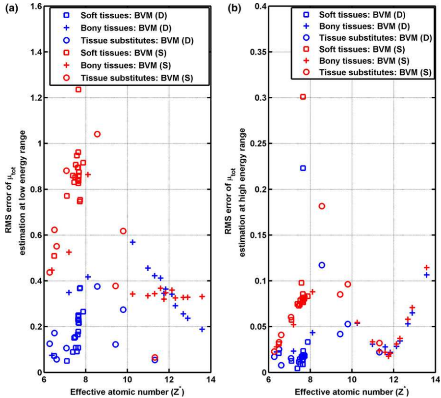
FIG. 7. RMS error of total cross-section estimates predicted by dBVM (double-basis pair) and sBVM (single-basis pair) for 43 tissues and phantom substitutes as functions of effective atomic number for the (a) low ( 20 \leq E \leq 50 keV) and (b) high ( 50 \leq E \leq 1000 keV) energy ranges. The thyroid tissue prediction error is outside the plotting range of the low-energy plot. [Color figure can be viewed at wileyonlinelibrary.com]
