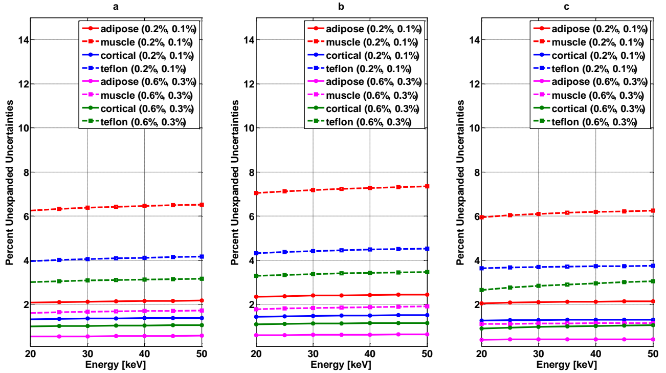
Figure S-F2. Percent unexpanded uncertainty of photoelectric coefficients for (a) tPFM, (b) vPFM and (c) BVM, respectively as functions of energy in the range 20 \leq E \leq 50 keV, at image intensity uncertainty levels (0.6%, 0.3%) and (0.2%, 0.1%) for (low, high) energy CT images. Four typical human tissues and tissue substitute were selected for analysis.
