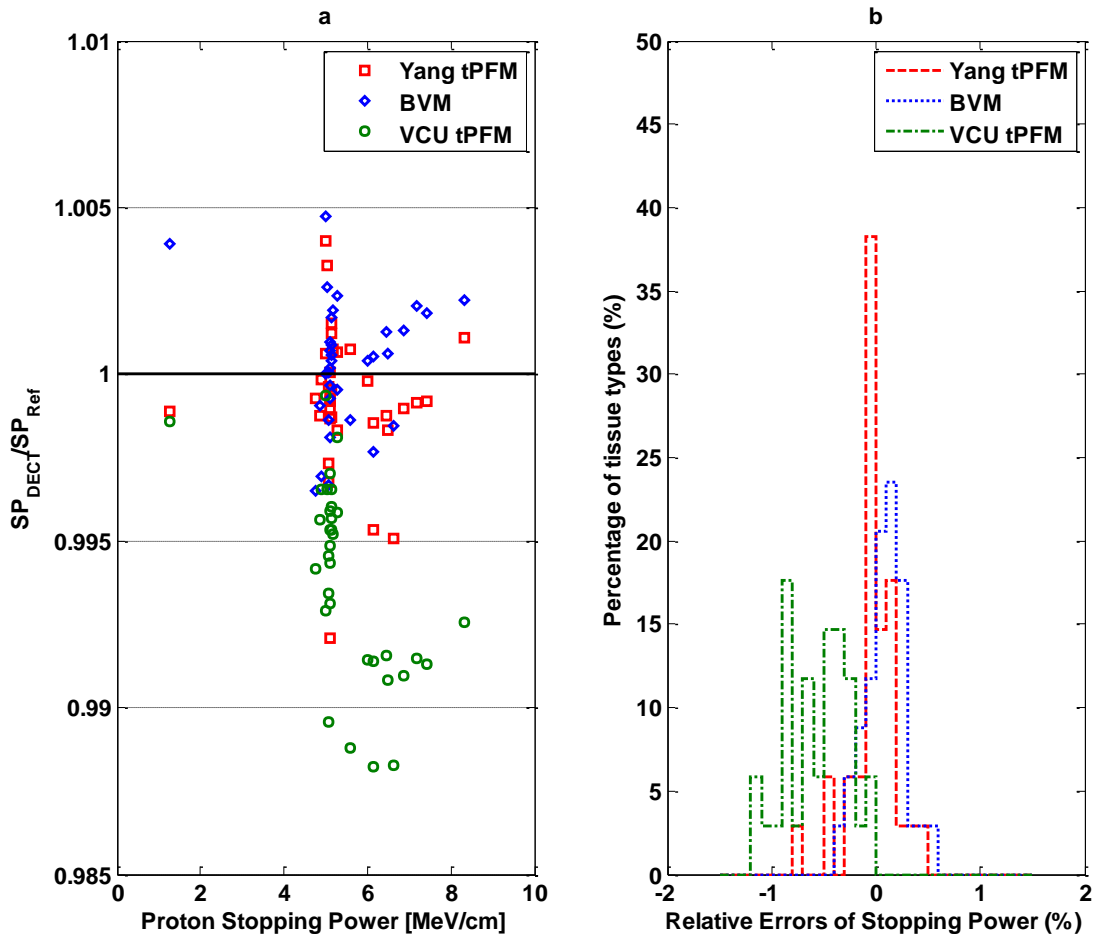
Fig. 2.5 (a) A comparison of errors in the stopping power predictions from different DECT models with reference values. The maximum relative error of prediction using the BVM was well below 0.5%. (b) The distribution of relative errors of the stopping power of 34 standard human tissues estimated by the BVM, Yang tPFM and VCU tPFM is shown.
