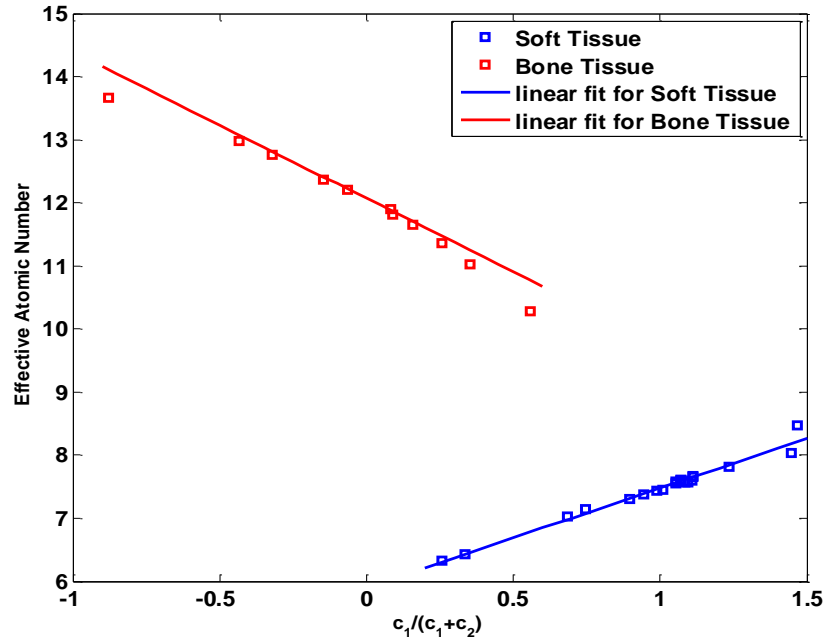
Fig.5.1 Linear correlation exists for Z^* and \alpha(\mathbf{x}) of ICRU tissues. The effective atomic number Z^* is computed from tPFM model, described in Ch.2.
