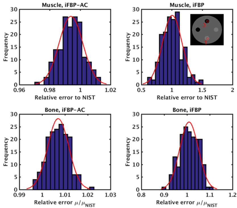
Fig. 5.16 Distribution of total linear attenuation bias at 28 keV for pixels within the muscle and cortical bone ROIs. The component images of iFBP-AC and iFBP are used. For a better visualization purpose, x-axis of each subplot uses different scales. The red circles represent the ROIs in each insert.
