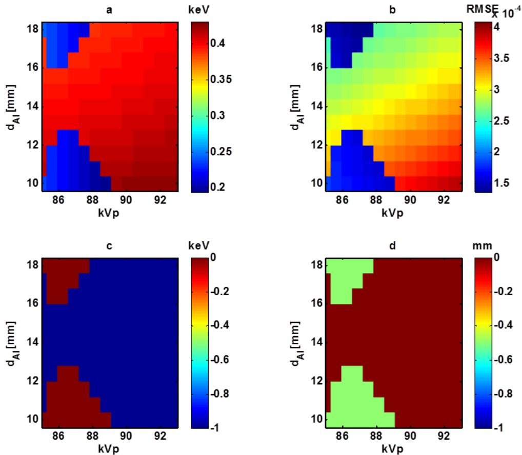
Fig.4.15 Comparisons of derived spectrum and independently simulated reference spectra for nominal 90 kVp with inherent filtration of aluminum ranging from 10 mm to 18 mm for the noiseless QF_{P,model} . The differences of mean energy (a), RMSE (b), kVp(c), and d_{Al} (d) are shown, respectively. Each pixel on the figures corresponded to the discrepancy for each candidate of reference spectrum.
