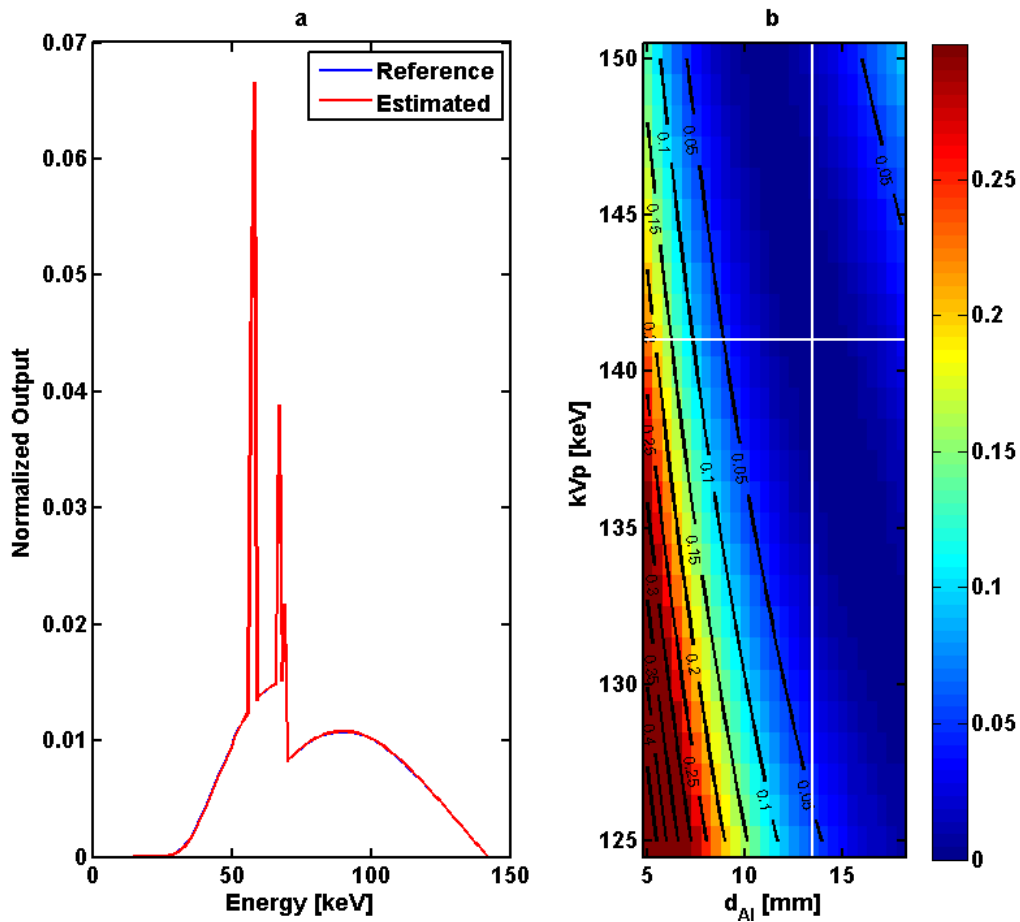
Fig.4.14 Comparison of derived spectrum and independent measured spectrum for 140 kVp of Y2 shown in (a), and the white cross in (b) corresponding to parameters for specifying a spectrum based on BM model.
