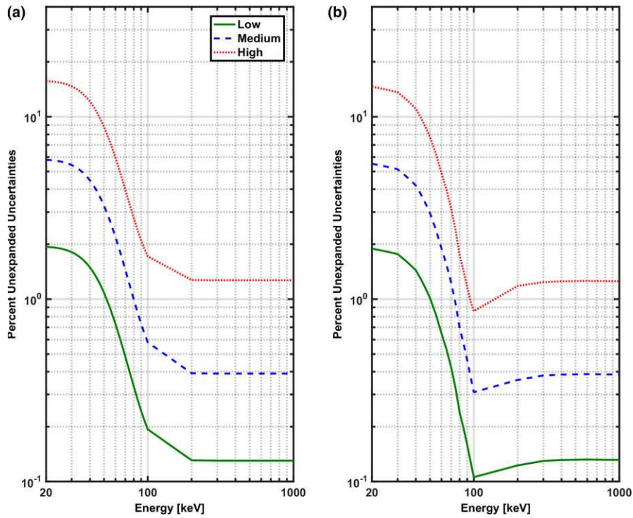
FIG. 6. Percent unexpanded uncertainty (coverage factor k = 1 ) of the linear energy-absorption coefficient for PMMA as a function of energy for the (a) tPFM and (b) BVM models. The low, medium, and high curves denoted the uncertainties corresponding to the (low, high) energy image-intensity uncertainties (0.2%, 0.1%), (0.6%, 0.3%), and (1.5%, 1.0%), respectively. [Color figure can be viewed at wileyonlinelibrary.com]
